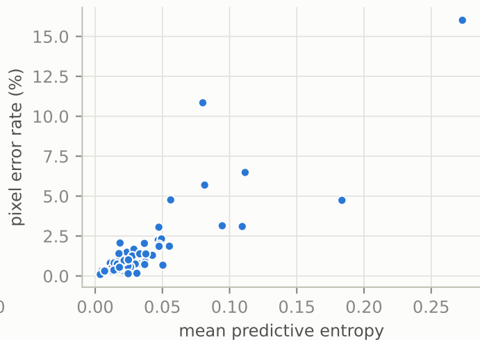
Per-image: entropy vs error ( r = 0.86 )
